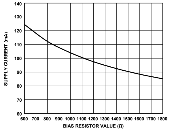
Figure 38. Supply Current vs. Bias Resistor Value
