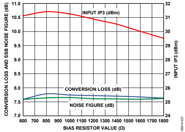
Figure 37. Power Conversion Loss, SSB Noise Figure, and Input IP3 vs. IF Bias Resistor Value
